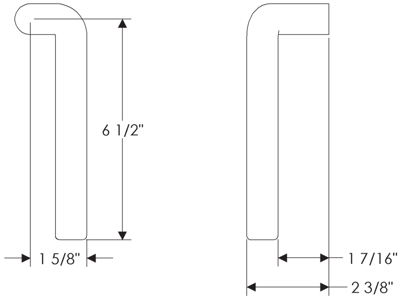
L177 Offset Tube Lever
