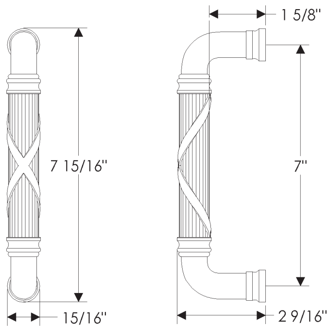
G626 7" Ribbon & Reed Grip Weight: 1.75 lbs.
