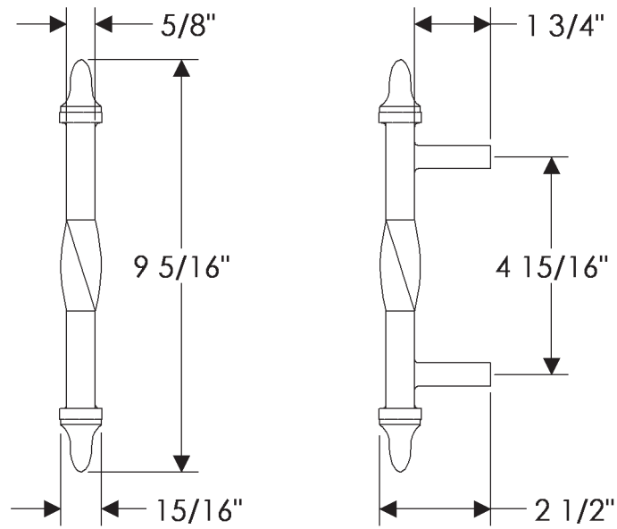
G621 4 15/16" Steeple Twist Grip Weight: 1.35 lbs.
