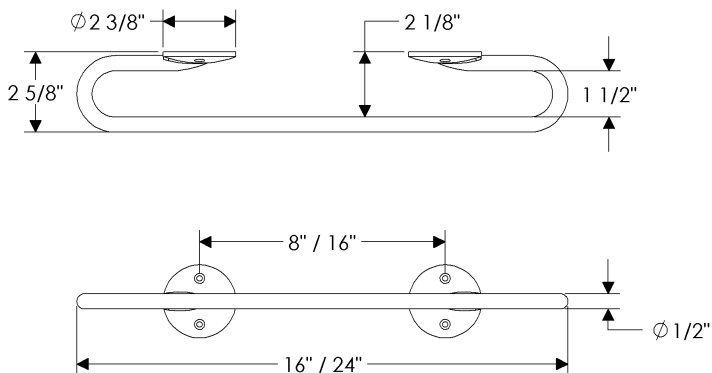
TB616, TB624 Cirque Towel Bar Cirque Collection
