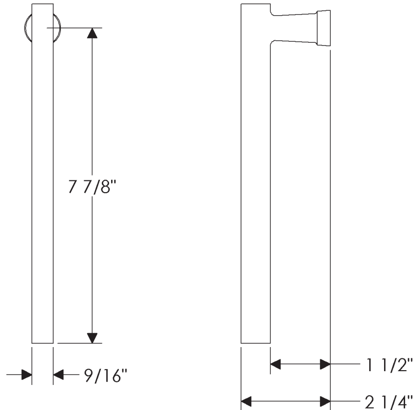
L264 Long Trolley Lever
