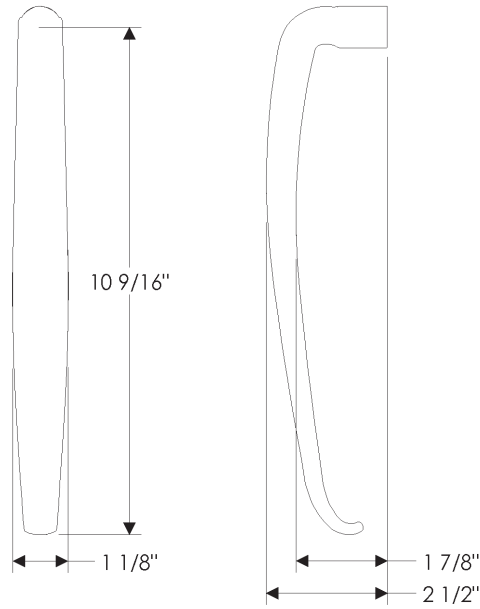
L144 Extra Long Hook Lever
