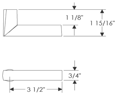
LW61 Mini Rail Lever Designed for WN window trim sets
