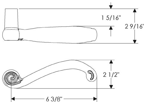
L156 Large Classic Scroll Lever Also available: L125 Classic Scroll Lever
