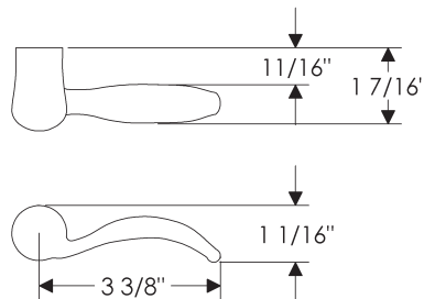
LW40 Mini Classic Lever Designed for WN window trim sets
