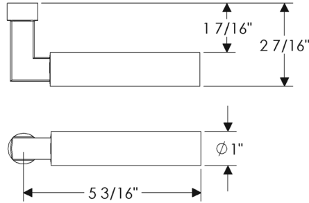
L154 Stalk Lever
