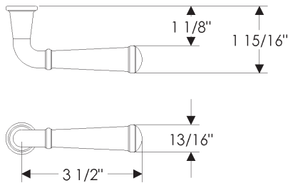
LW60 Mini Harrington Lever • Designed for WN window trim sets
