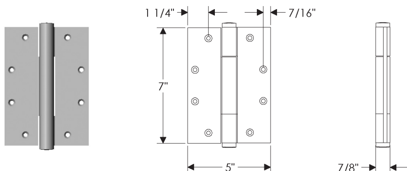
HNG7x5 Concealed Bearing Hinge
