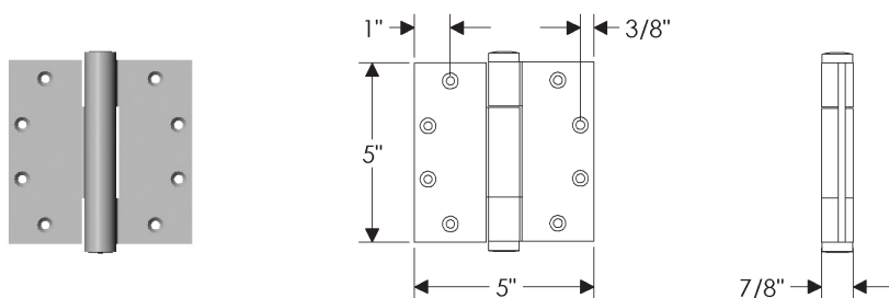
HNG5 Concealed Bearing Hinge
