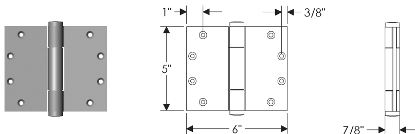
HNGWT5x6 Concealed Bearing Hinge
