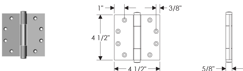
HNG4.5A Concealed Bearing Hinge
