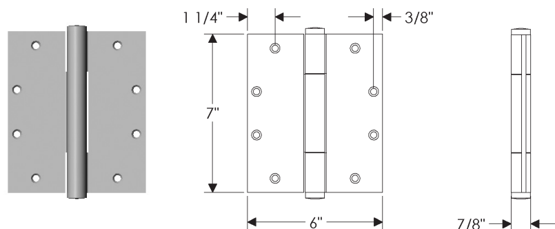
HNG7x6 Concealed Bearing Hinge
