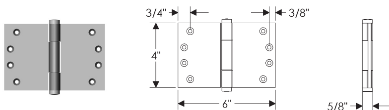
HNGWT4x6A Concealed Bearing Hinge
