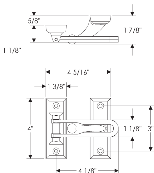
DG1 Door Guard
