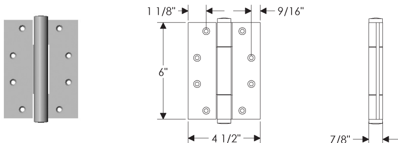
HNG6x4.5 Concealed Bearing Hinge
