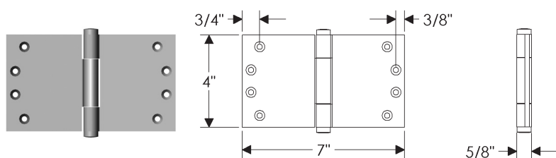
HNGWT4x7A Concealed Bearing Hinge
