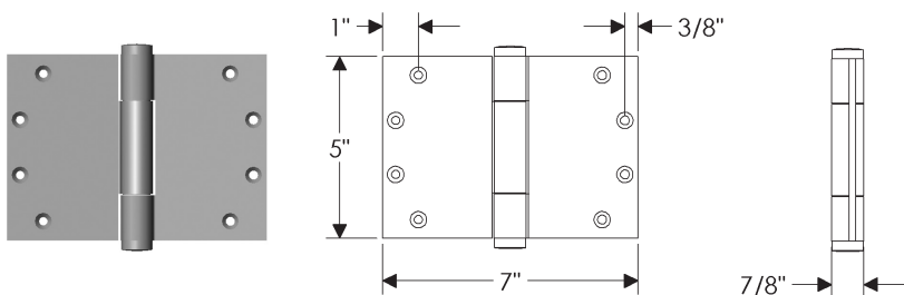
HNGWT5x7 Concealed Bearing Hinge
