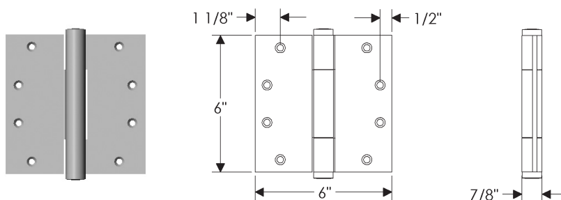
HNG6 Concealed Bearing Hinge
