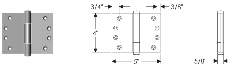
HNGWT4x5A Concealed Bearing Hinge
