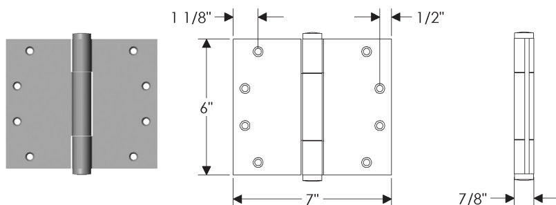
HNGWT6x7 Concealed Bearing Hinge
