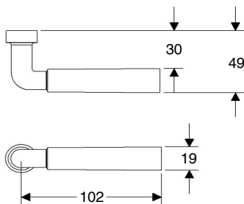
LB70 Small Coupler Lever
