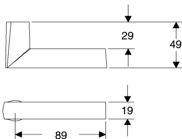
LB61 Small Rail Lever
