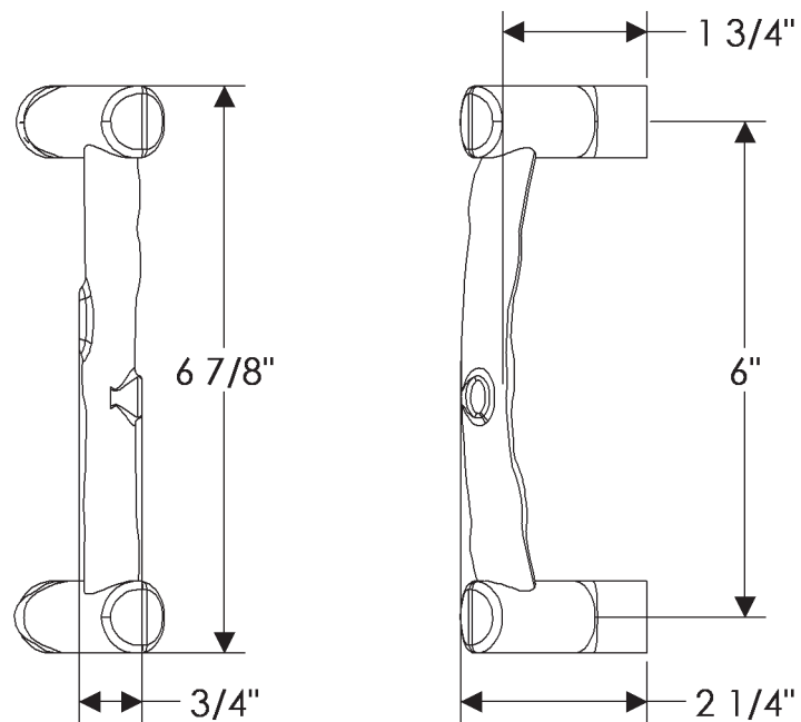
SDT6 6" Offset Branch Grip Weight: 1.50 lbs.
