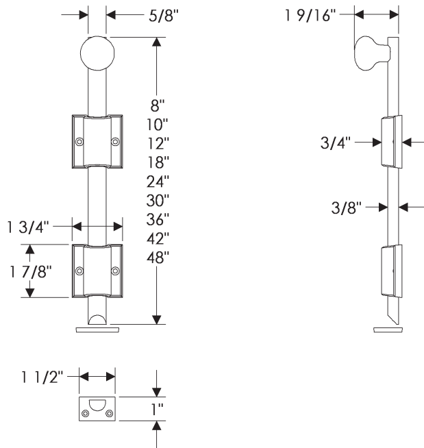
MB8 Surface Bolt, Rectangular Mounting Brackets
