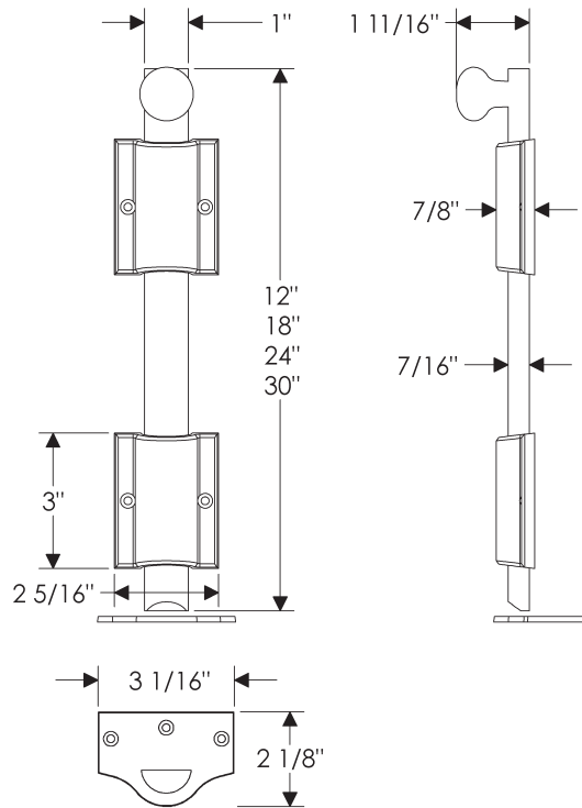
MB7 Surface Bolt, Rectangular Mounting Brackets
