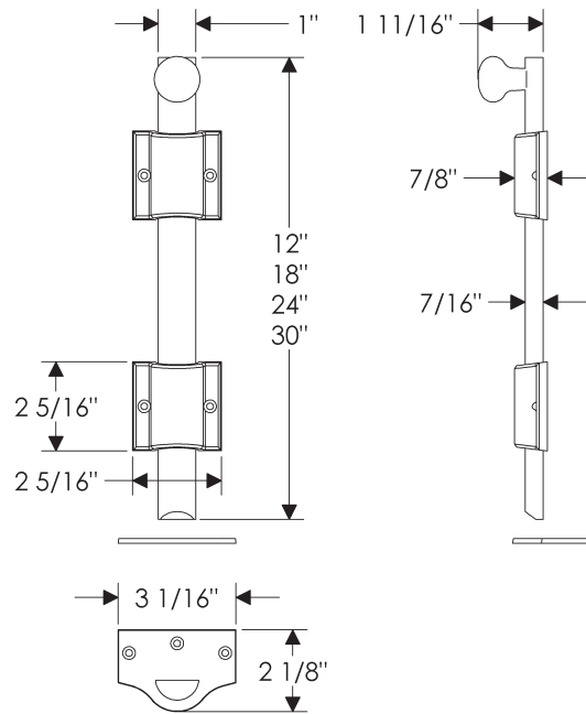
MB2 Surface Bolt, Square Mounting Brackets
