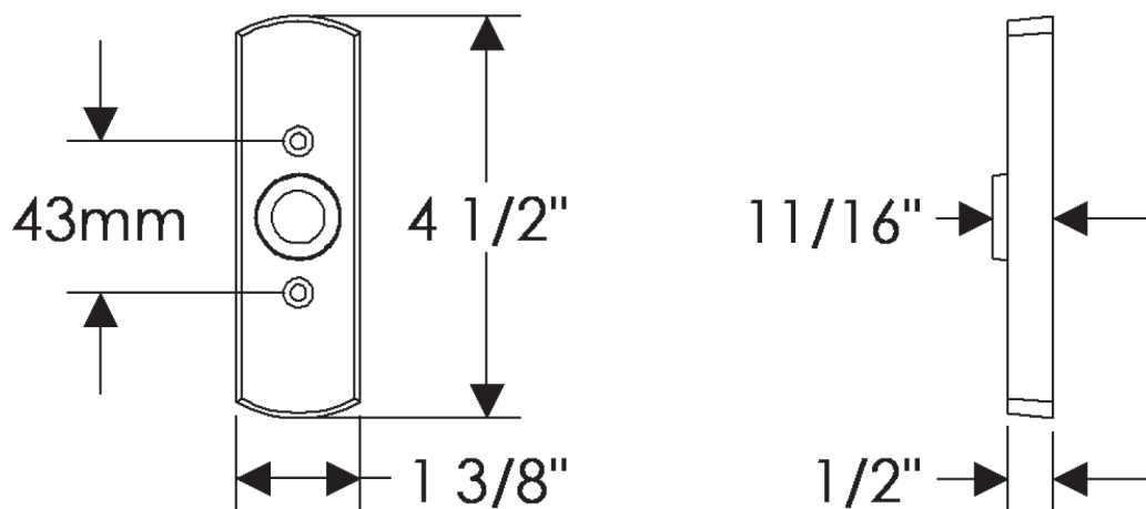
EW501 Curved Window Escutcheon 1\frac{3}{8}" \times 4\frac{1}{2}"
