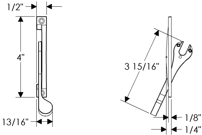
WL180 Sash Lock
