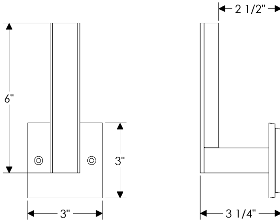
TP30310 Trousdale Vertical Toilet Paper Holder Trousdale Collection
