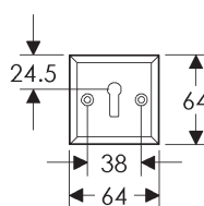
SL416/BK418 Minimum C-C 61mm
