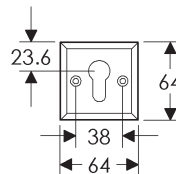
SL416/EU418 Minimum C-C 61mm
