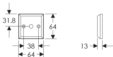
SL416/BL418 Minimum C-C 68mm
