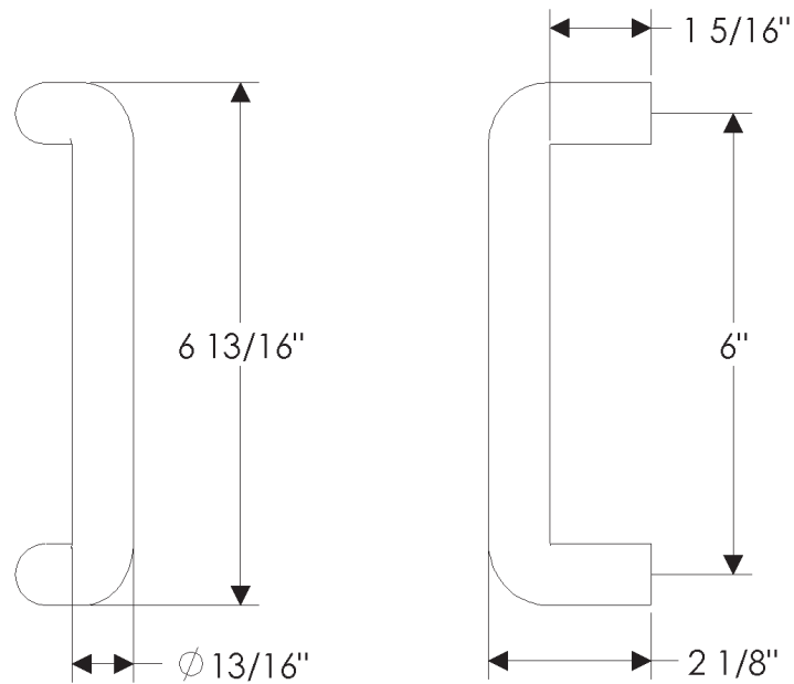
SDP6 6" Offset D Grip Weight: 1.45 lbs.
