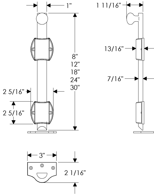
MB1 Surface Bolt, Oval Mounting Brackets
