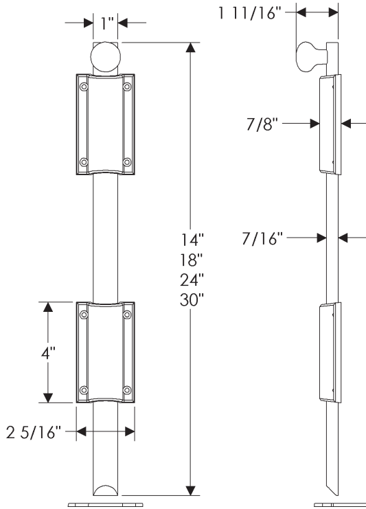
MB12 Surface Bolt, Rectangular Mounting Bracket
