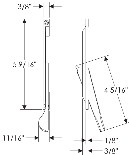
LC600 Sash Lock Designed for Truth Encore Multi-point Casement Locks
