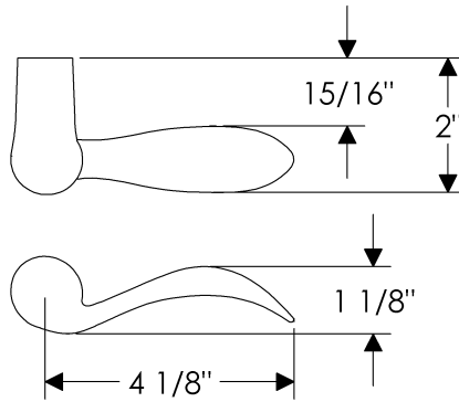
LB50 Small Beaver Tail Lever
