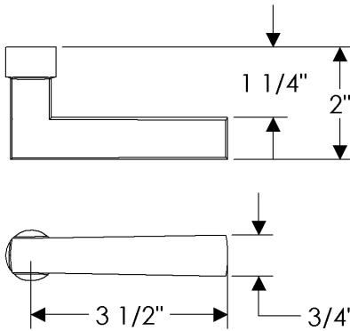
LB30 Small Reed Lever
