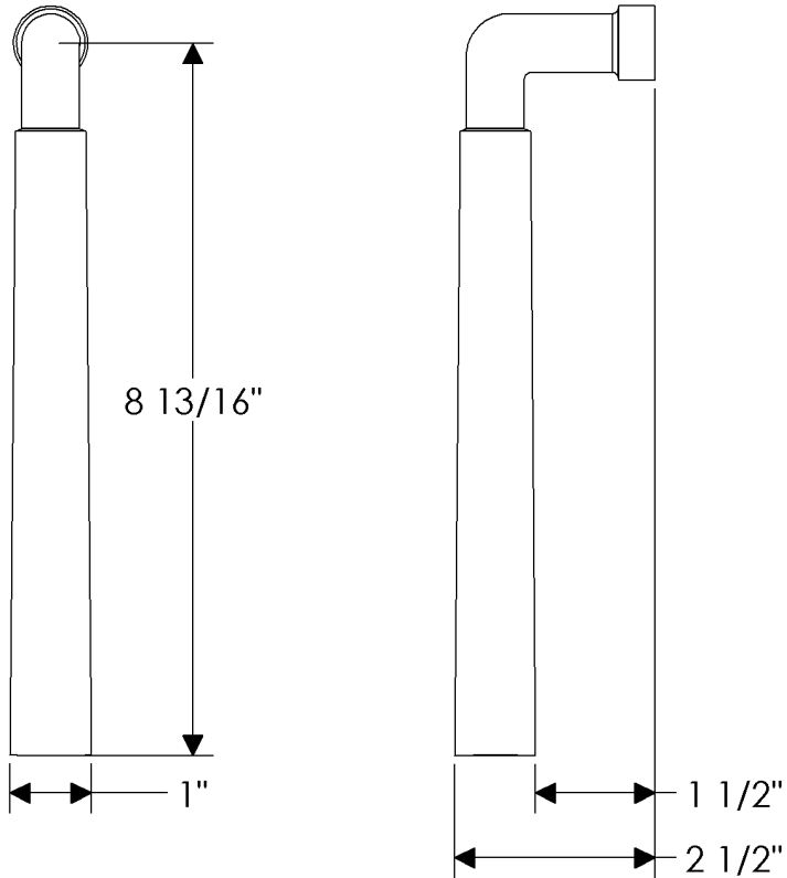
L331 Long Coupler Lever
