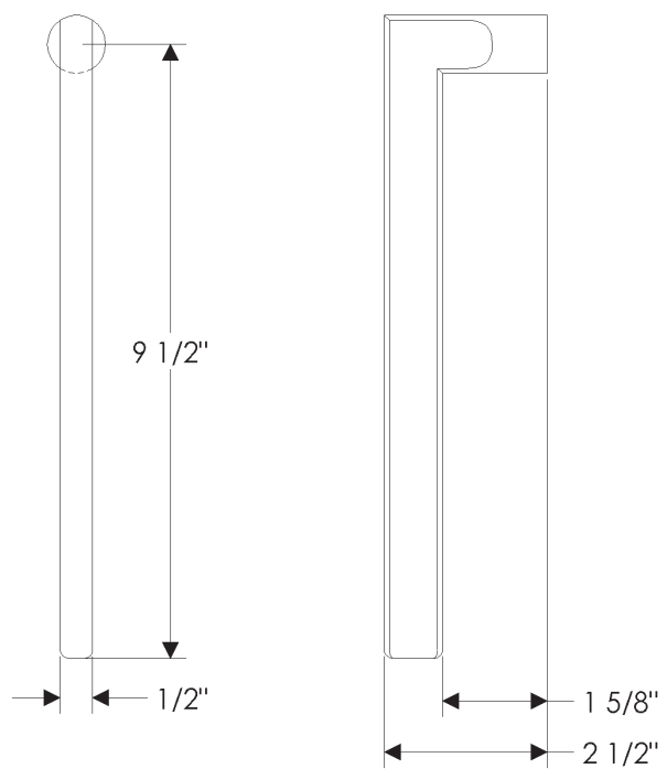
L145 Long Olympus Lever
