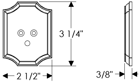
IP30890
