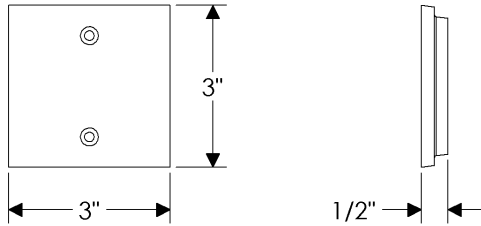
IP30390 Trousdale Escutcheon Trousdale Collection 3" x 3"
