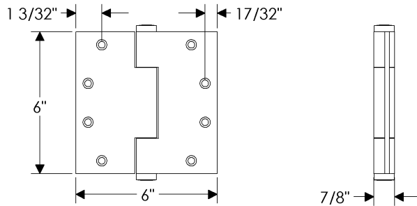
HNG6 Concealed Bearing Hinge 6" x 6"
