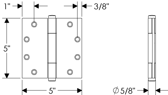
HNG5A Butt Hinge 5" x 5"
