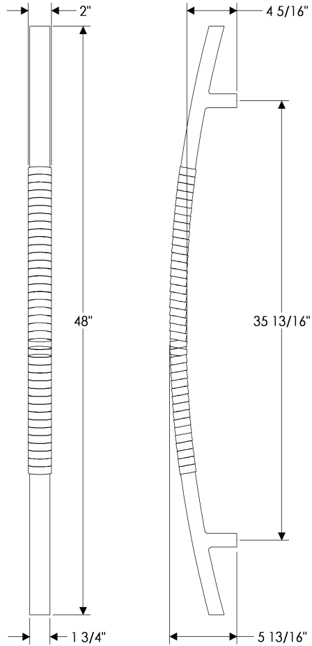
G670 35 3/16" Lariat Grip 31.75 lbs.
