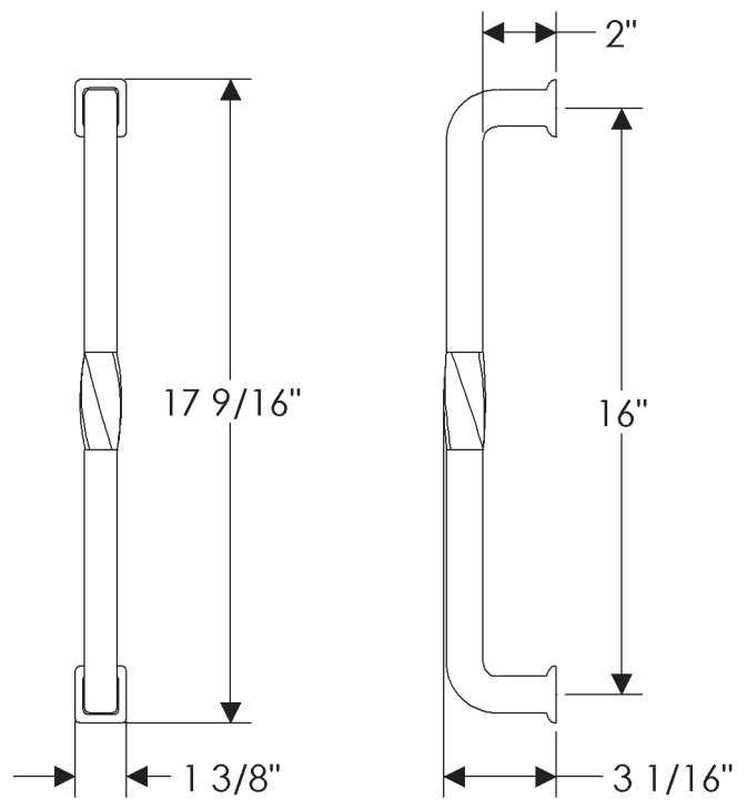
G669 16" Sash Twist Grip Weight: 5.30 lbs.
