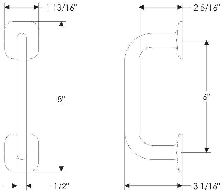
G615 6" Sash Grip Weight: 1.45 lbs.
