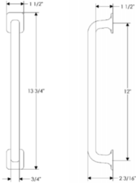
G612AP Sash Appliance Pull
