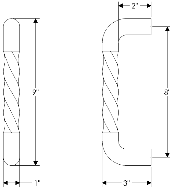
G605 8" Twisted D Grip Weight: 9.75 lbs
