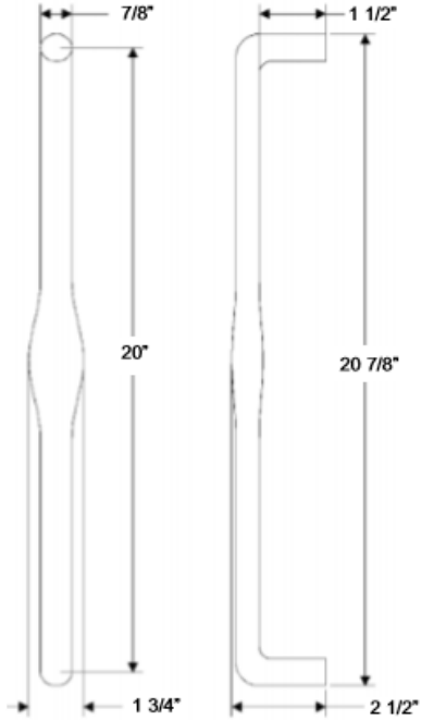
G372AP Provence Appliance Pull
