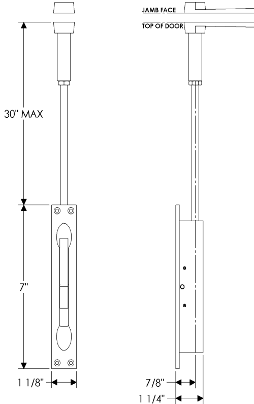
FB105 Edge Mount Flush Bolt
