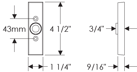
EW225 Metro Escutcheon 1 1/4" x 4 1/2"
