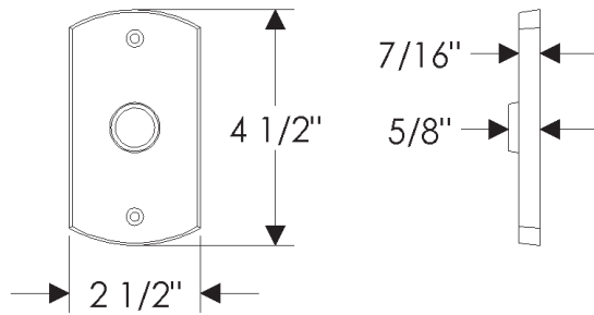
E504 Curved Escutcheon 2 1/2" x 4 1/2"
