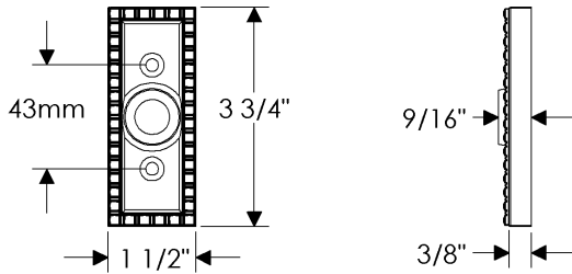
EW30700 Corbel Rectangular Escutcheon 1 1/2" x 3 3/4"
