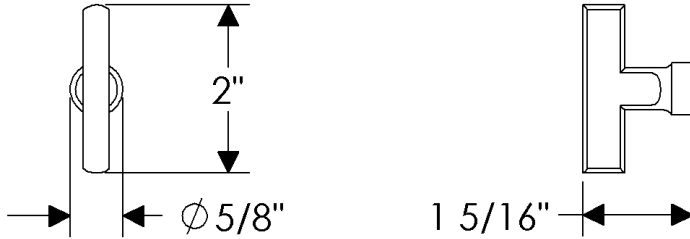
CK199 Olympus Cabinet Knob
