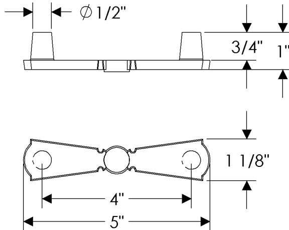
CK10050 Paris Cabinet Pull, 4" Roger Thomas Collection
