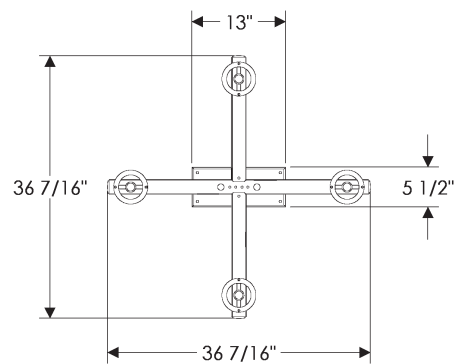
C450 Cross Arm Chandelier with Round Glass 36 7/16" x 36 7/16" x 8"
