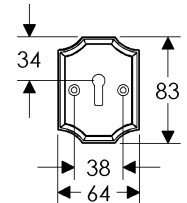
SL30805/BK30890 Minimum C-C 114mm
