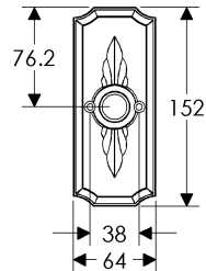
SL30805/BL30890 Minimum C-C: 120mm
