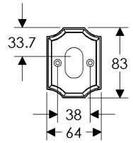
SL30805/OC30890 Minimum C-C: 114mm
