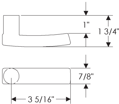
LW37 Mini Strap Lever Designed for WN window trim sets
