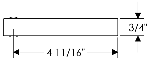
L303 Boiler Lever
