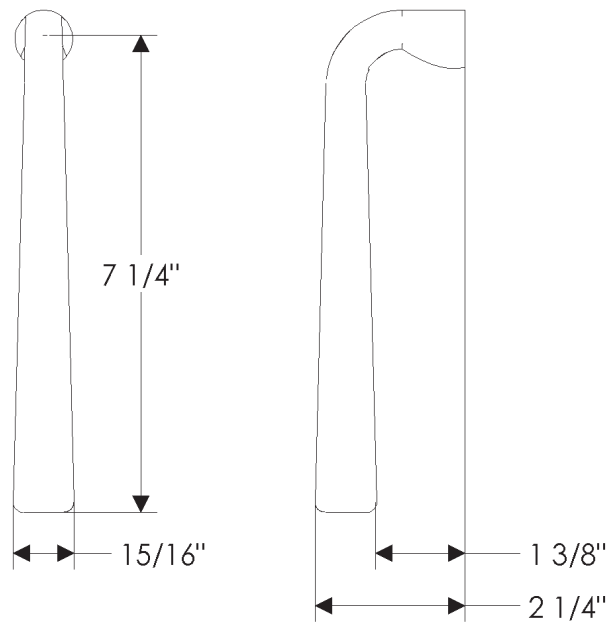
L148 Long French Lever
