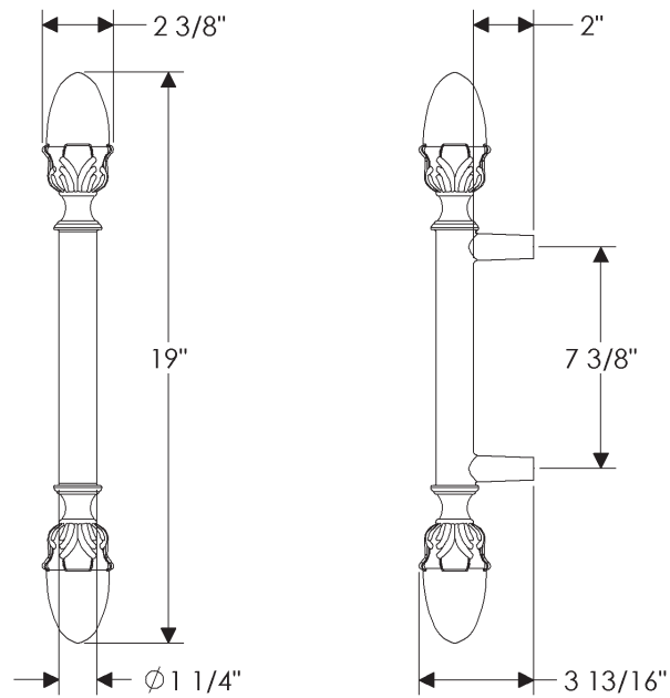
G660 7 3/8" Acorn Grip Weight: 10.75 lbs.
