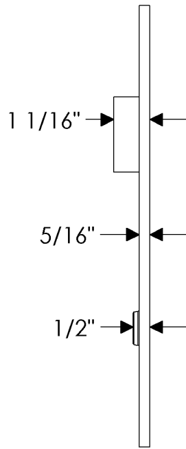
1-3/8" - 2-3/8" DOOR THICKNESS
