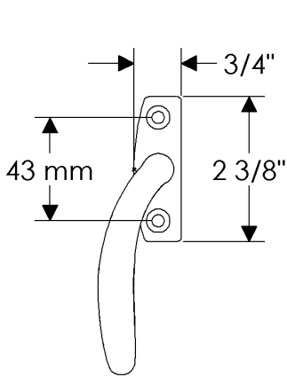
WL210 Sash Lock Left hand shown
