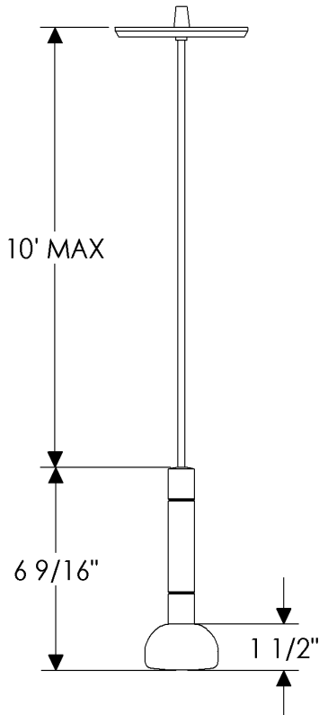
PE625 Torch Pendant 1 \frac{1}{2} " x 2 \frac{1}{2} " x 6 \frac{9}{16} "
