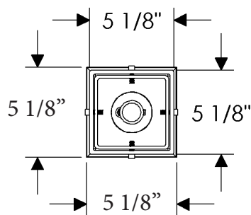
PE425 Foxtrot Pendant 5 1/8" x 5 1/8" x 13 3/4"
